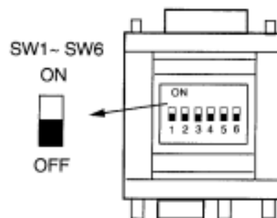
VGA/MAC ADAPTER
