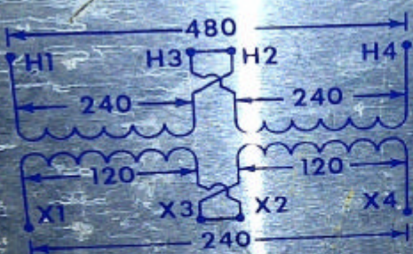
SERIES CONNECTION
