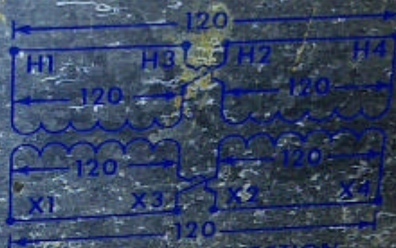
PARALLEL CONNECTION
